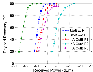
Fig. 4. Packet recovery for buffered and converted payloads from channel A.
