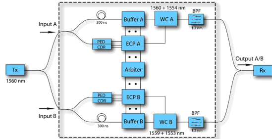
Fig. 1. Buffers, wavelength converters, and electronic lookup of a 2x2 optical packet switch
