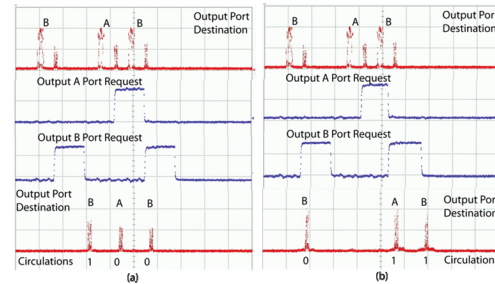
Fig. 2. Input packet stream, port request signals, and buffered payloads (a) channel A (b) channel B
