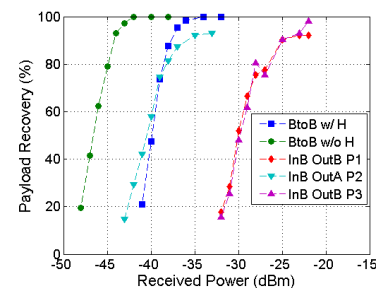
Fig. 5. Packet recovery for buffered and converted payloads from channel B.
